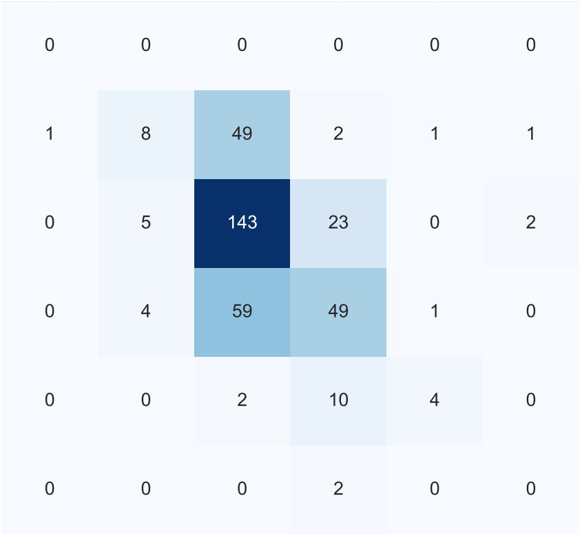
SARIMA (meteo) — test Exact: 55.7% ±1: 96.2% QWK: 0.379
